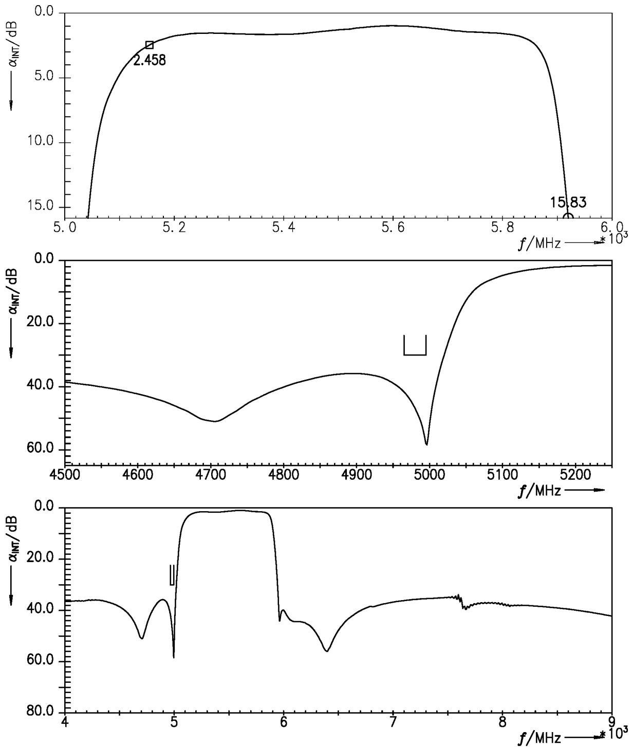
Figure 5: Attenuation (LTE) (integration window = 10 MHz).
