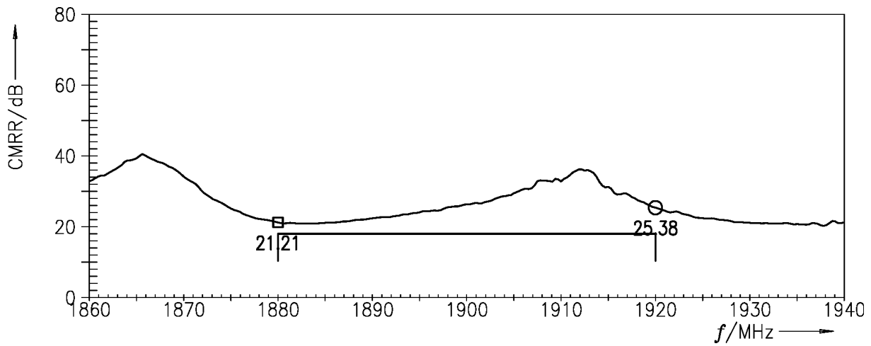
Figure 7: Common-mode rejection ratio.
