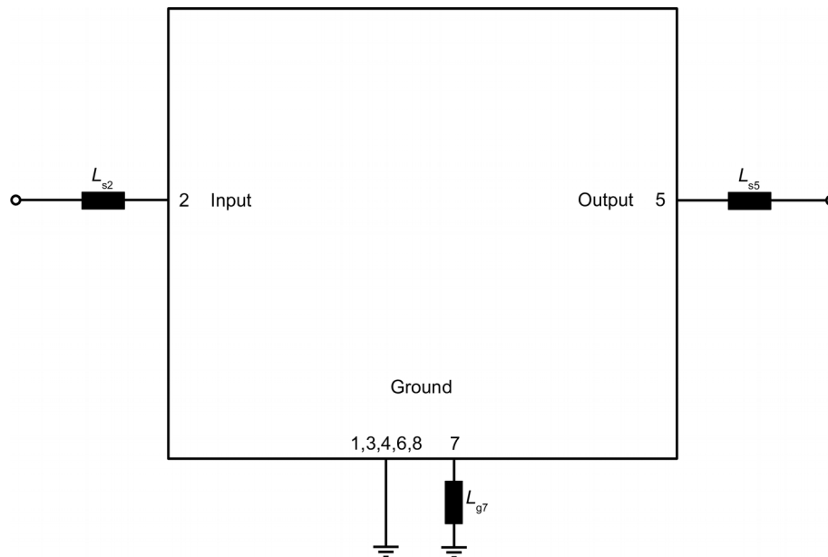
Figure 3: Schematic of matching circuit.
