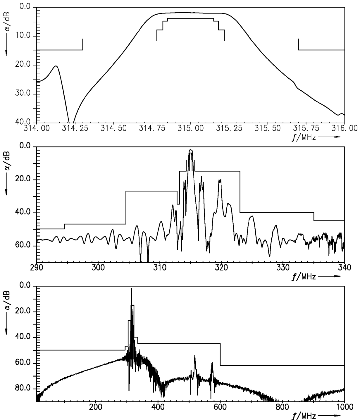
Figure 5: Attenuation.
