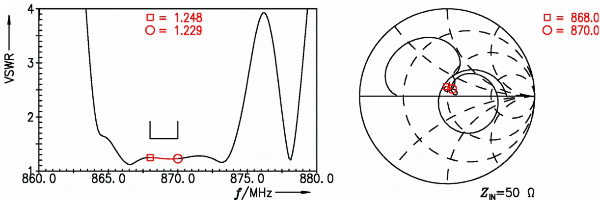
Figure 4: Reflection coefficient at IN port.
