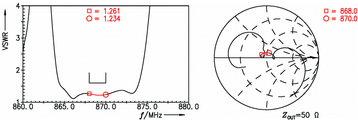
Figure 5: Reflection coefficient at OUT port.
