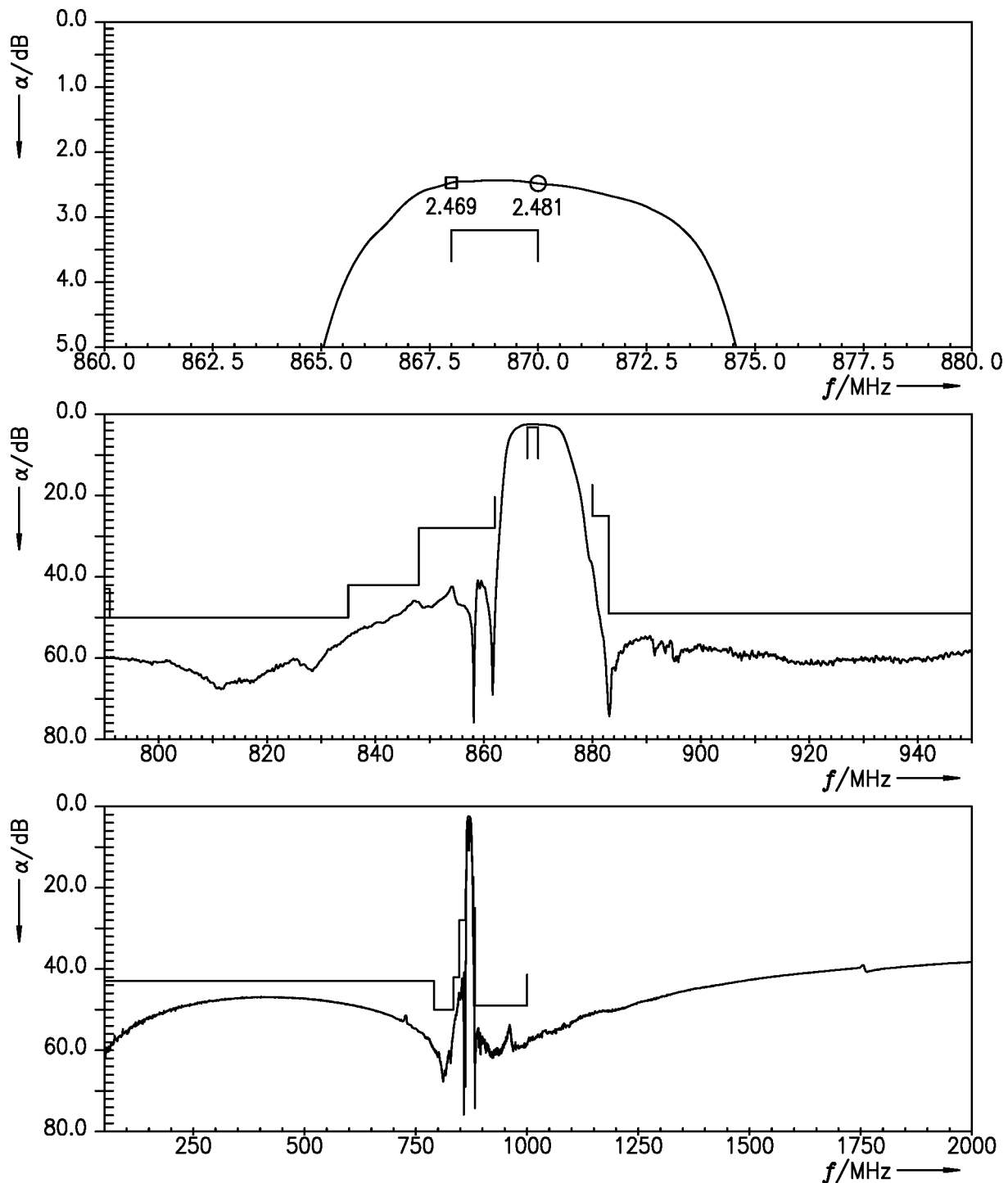
Figure 3: Attenuation.
