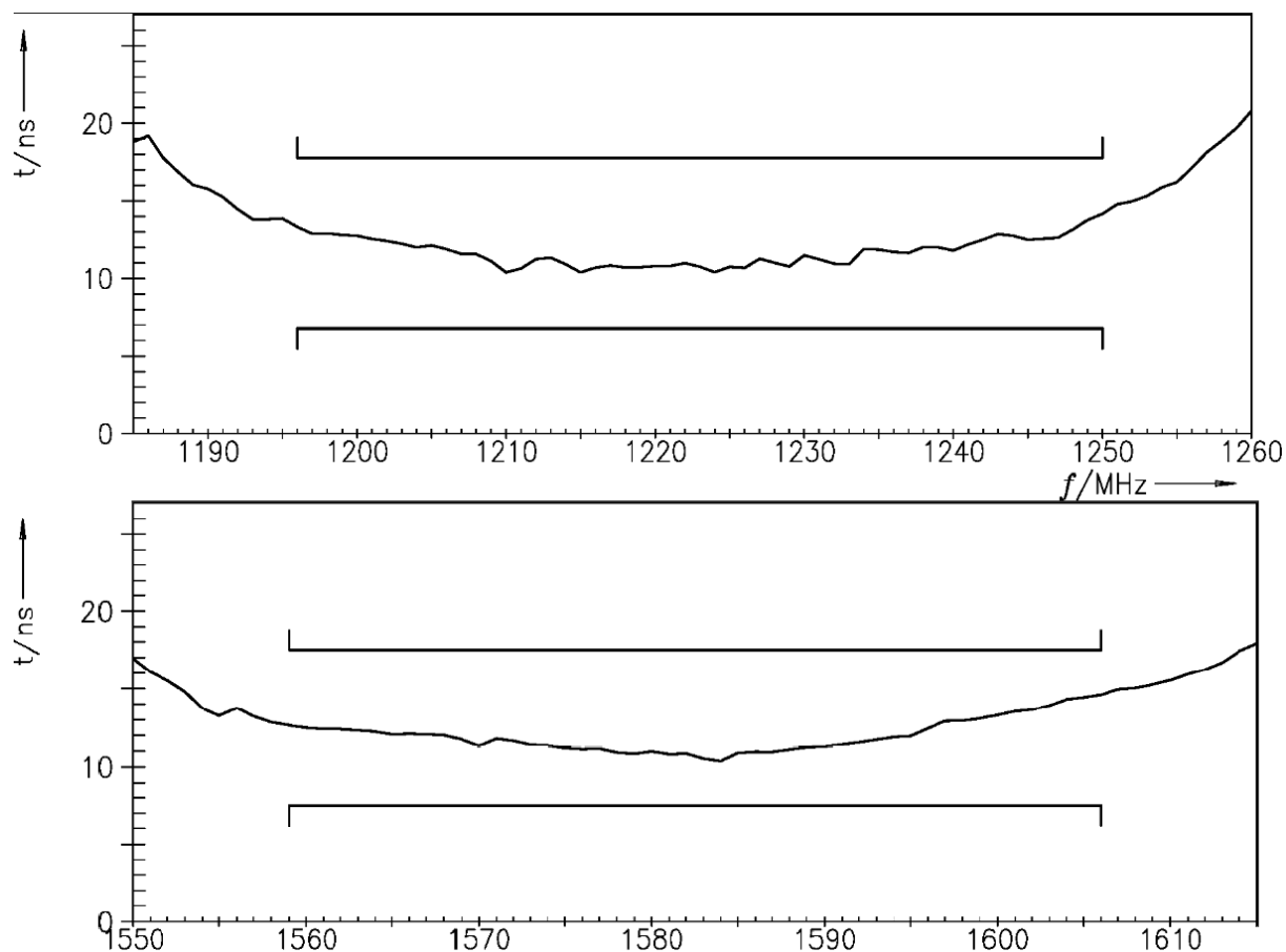
Figure 7: Group delay ripple.
