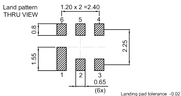
Figure 1: Drawing of package. See Sec. Package information (p. 18).
