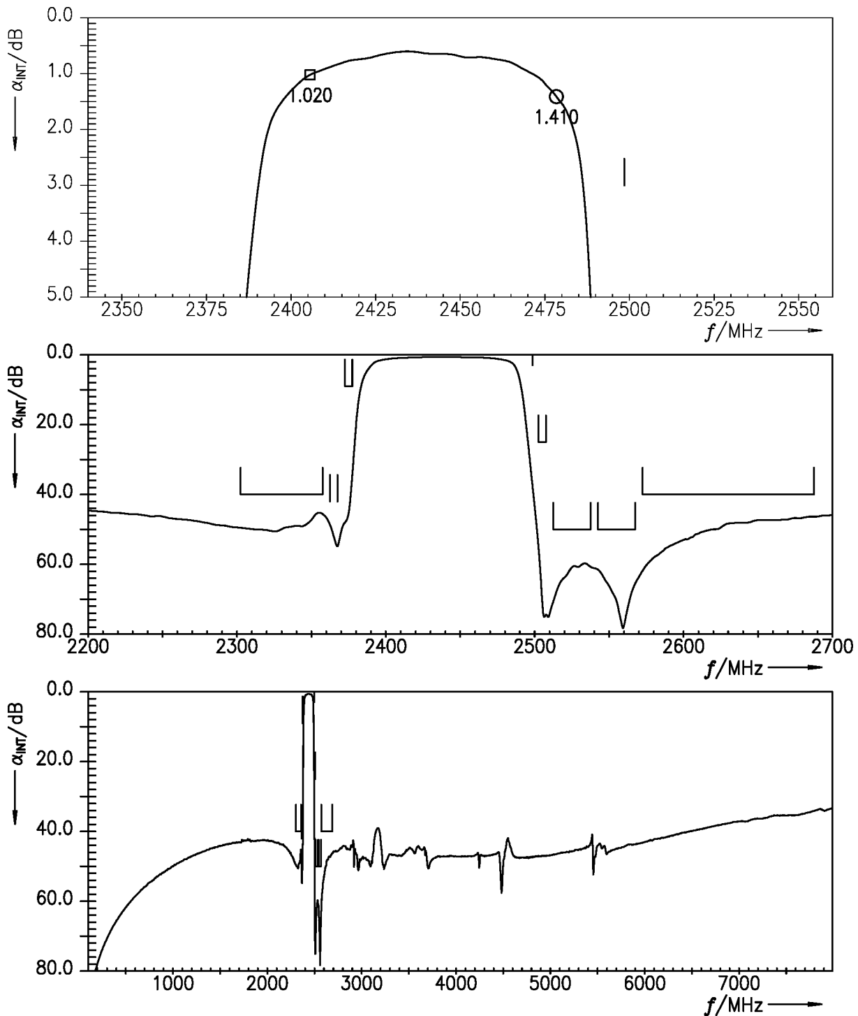
Figure 7: Integrated attenuation (integration window = 5 MHz).
