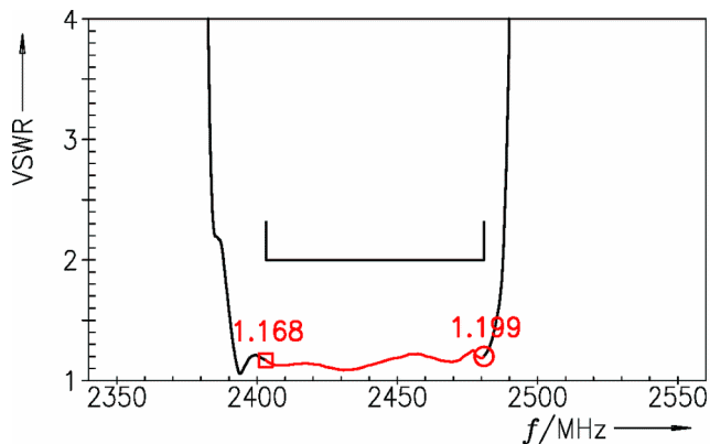
Figure 8: Reflection coefficient at input port.
