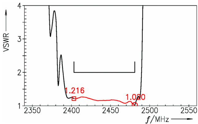
Figure 9: Reflection coefficient at output port.
