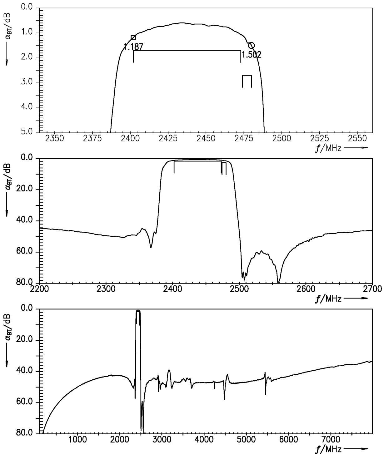
Figure 6: Attenuation (BT) (integration window = 1.0 MHz).
