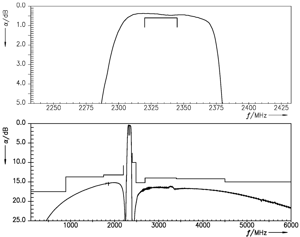
Figure 4: Attenuation.
