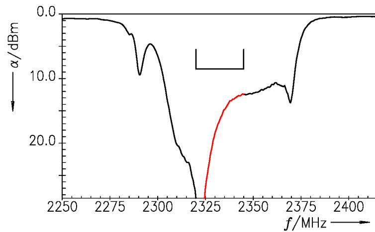
Figure 6: Return loss at output port.
