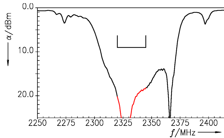
Figure 5: Return loss at input port.
