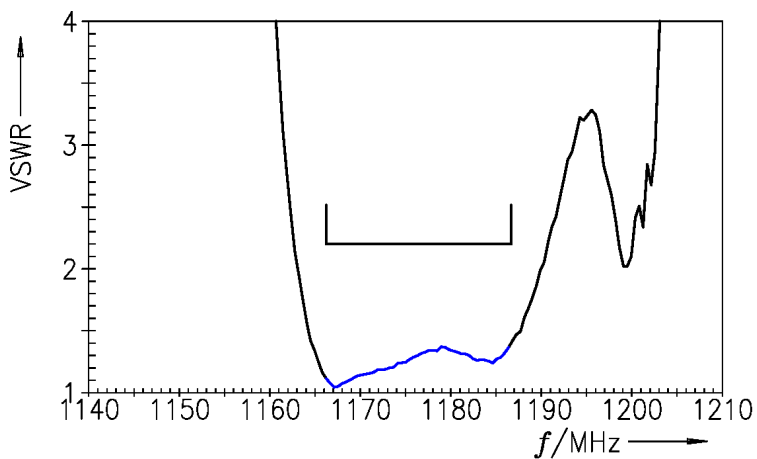
Figure 5: Reflection coefficient at GPS L5 port.
