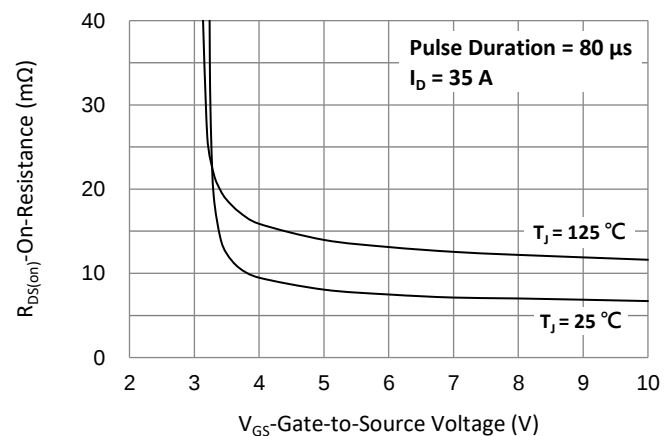
Fig.6 On-Resistance vs. Gate-Source Voltage
