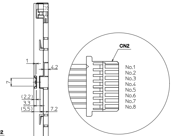
DETAIL B (5:1)
