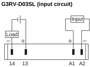
Terminal Arrangement/ Internal Connection Diagram (TOP VIEW)
