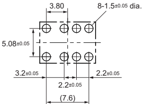
Mounting Dimensions (TOP VIEW)
