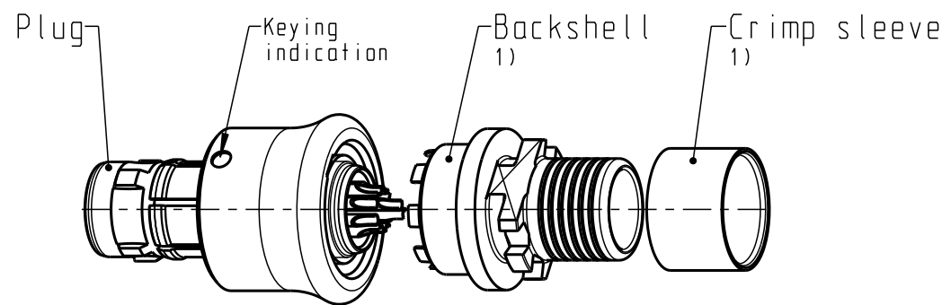
Delivery condition 2:1
