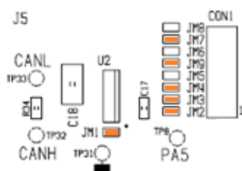
8-pin CAN operation
