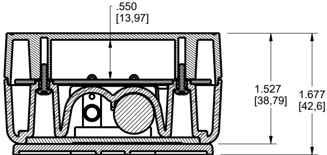
SECTION S-S
