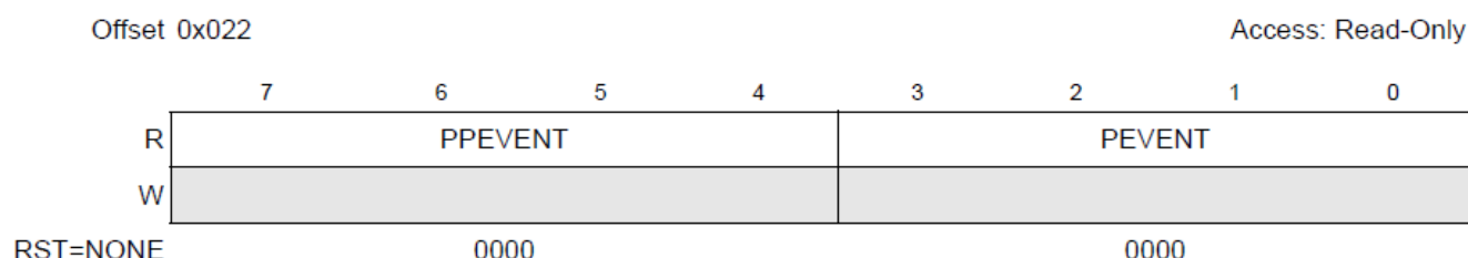
Figure 3-15. PWR_EVENT Register
