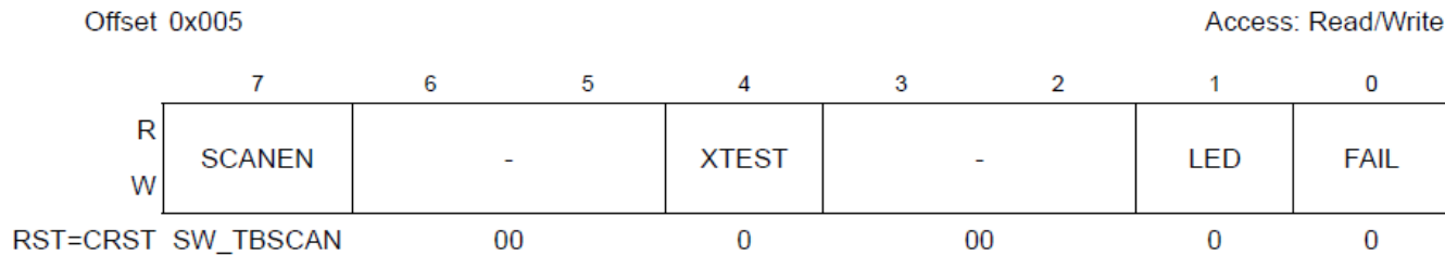
Figure 3-6. CTL Register
