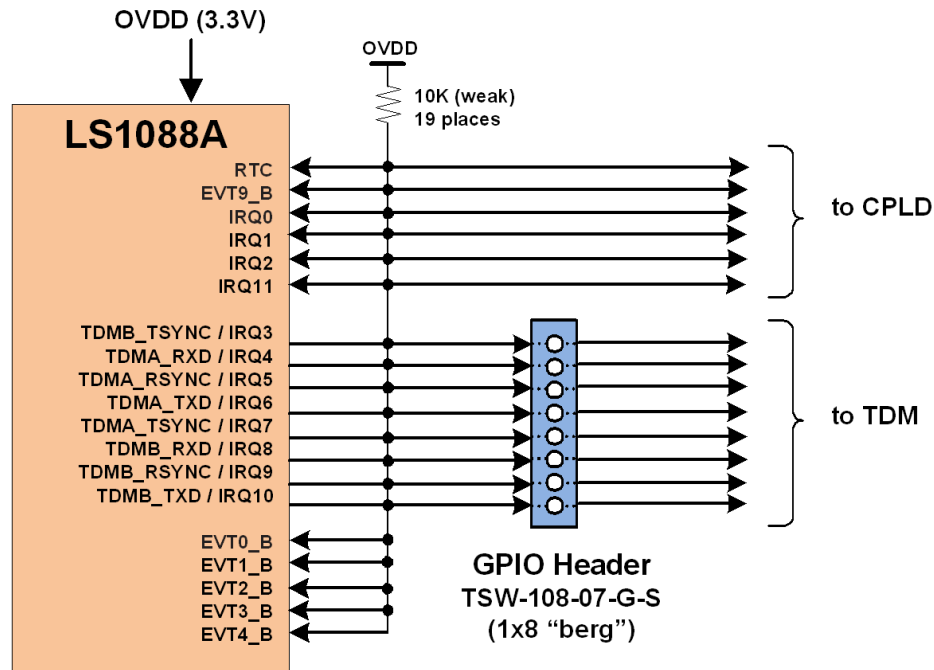
Figure 2-27. GPIO interface
