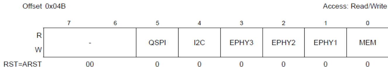
Figure 3-29. RST_MASK1 Register
