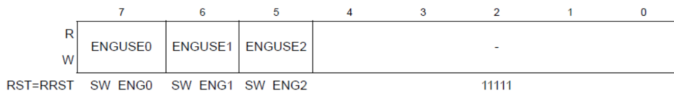
Figure 3-42. DUTCFG11 Register
