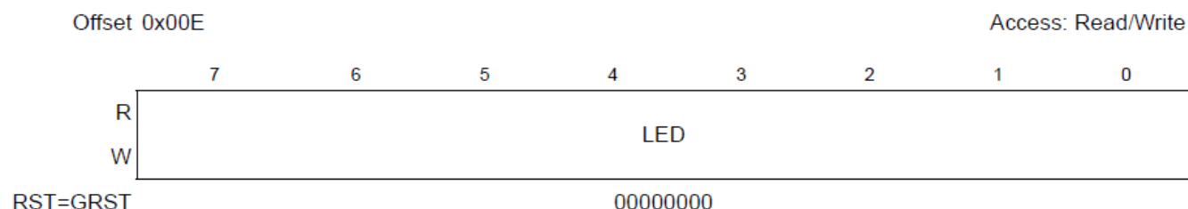
Figure 3-12. LED Register
