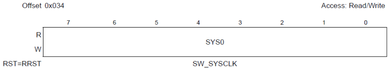
Figure 3-21. SYSCLK_D0 Register
