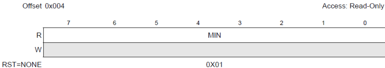
Figure 3-5. MINOR Register
