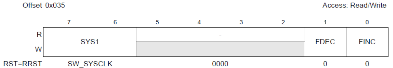
Figure 3-22. SYSCLK_D1 Register
