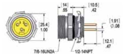
Male Receptacles
