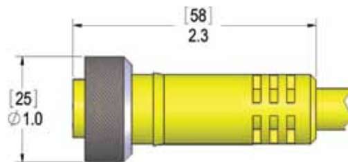
Straight Plug
