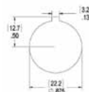
Cut-out
