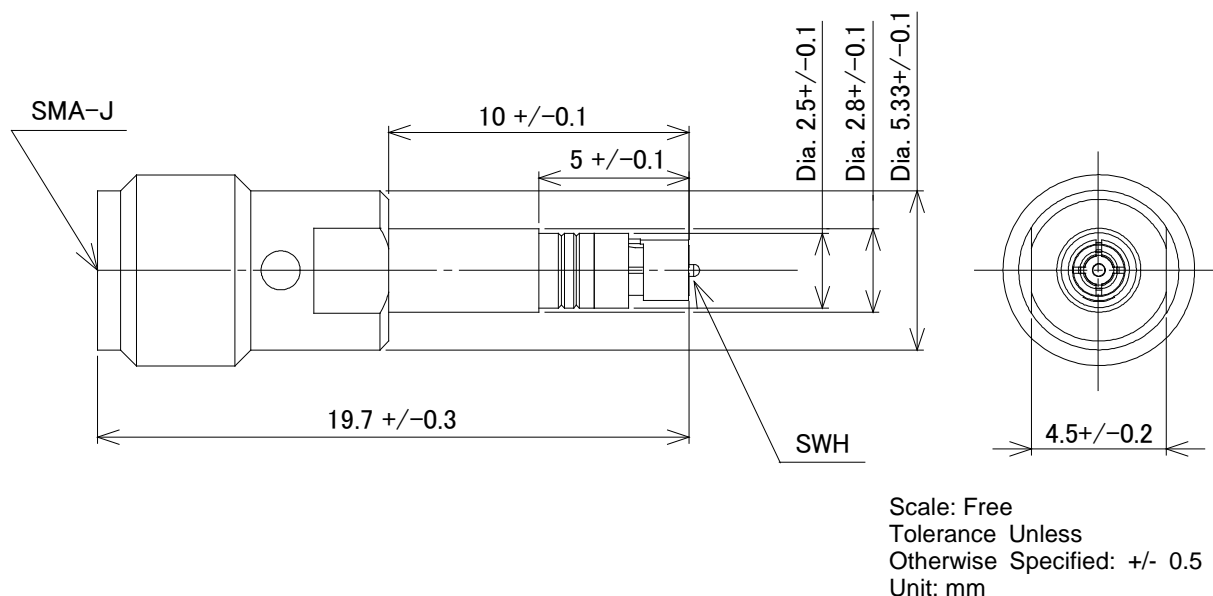
Figure 1 Construction
