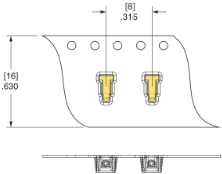
0986-X-58 Tape & Reel Details
