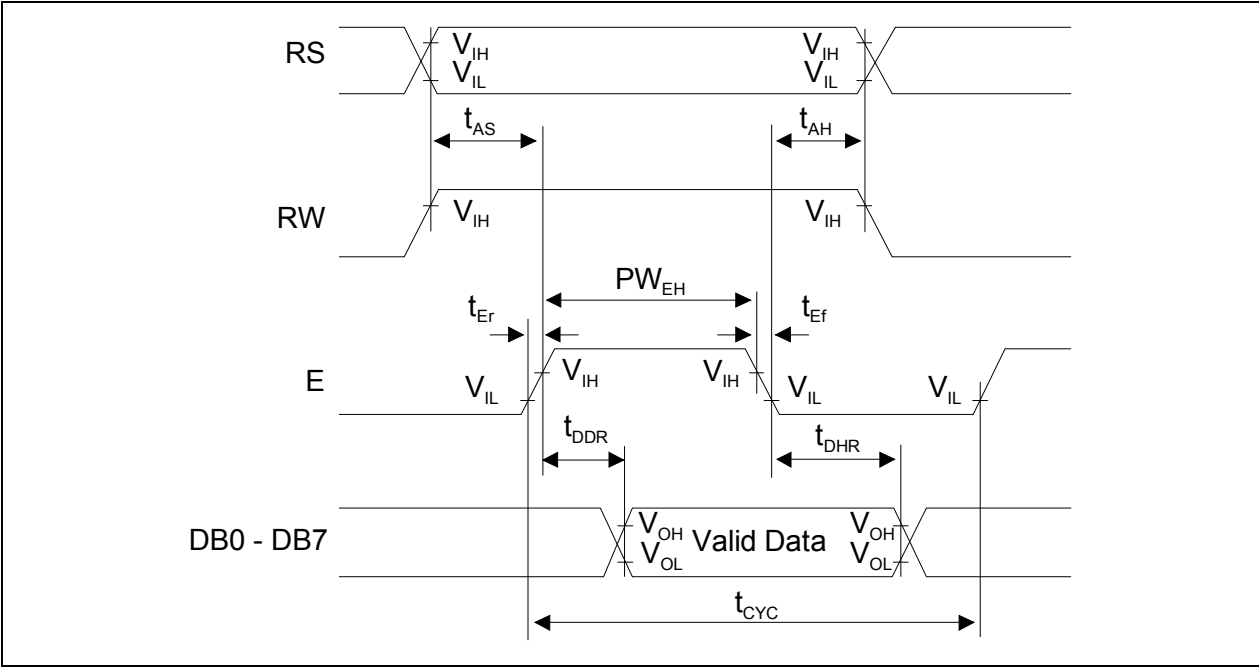
Fig.2 Read Operation Timing
