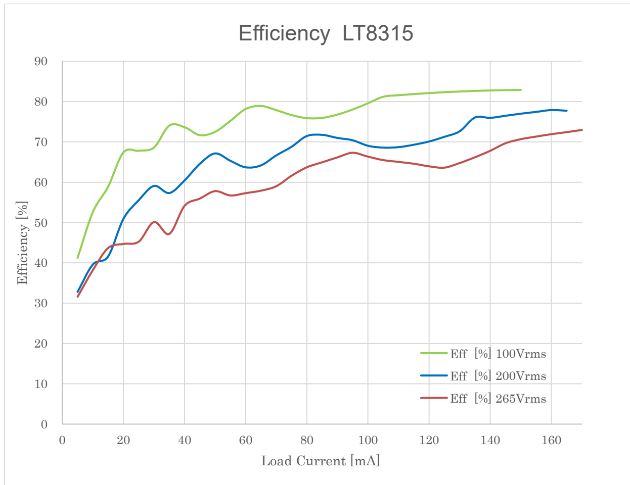
Figure 8.2.1-1 Efficiency
