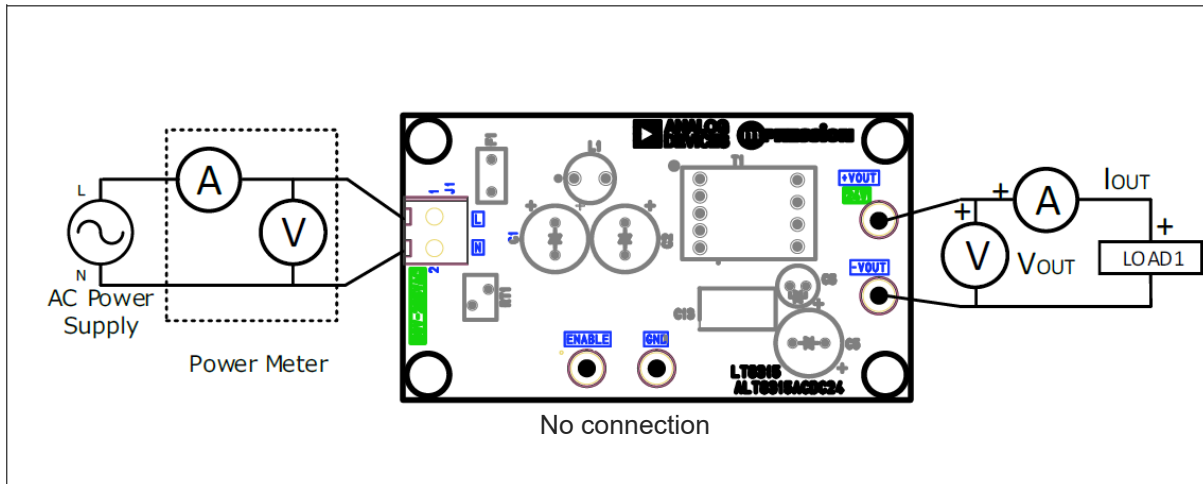
Figure 7-1 Measuring Circuit
