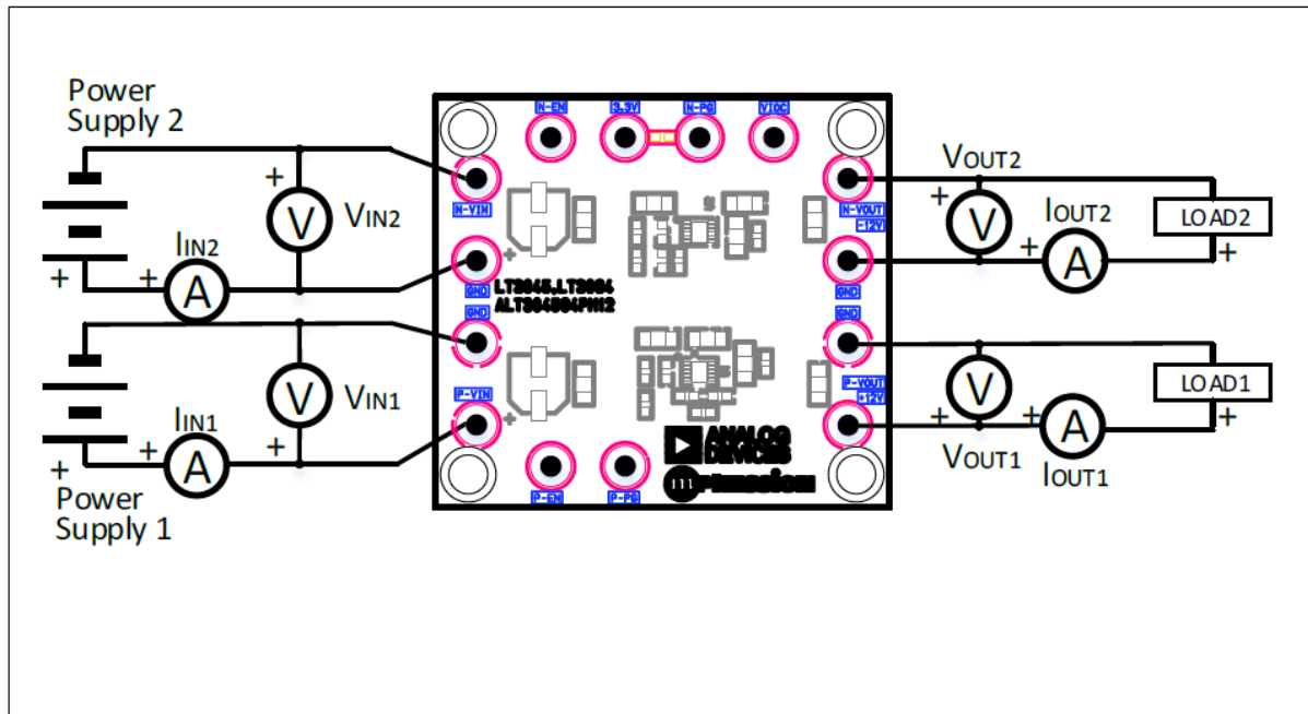
Figure 7-1 Measuring Circuit
