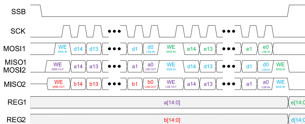
Figure 21. SPI Read & Write (2 ICs Daisy-chained)
