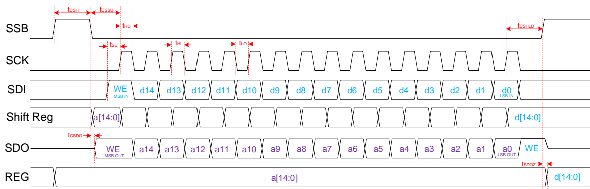
Figure 18. SPI Read & Write (1 IC, No Daisy Chain)
