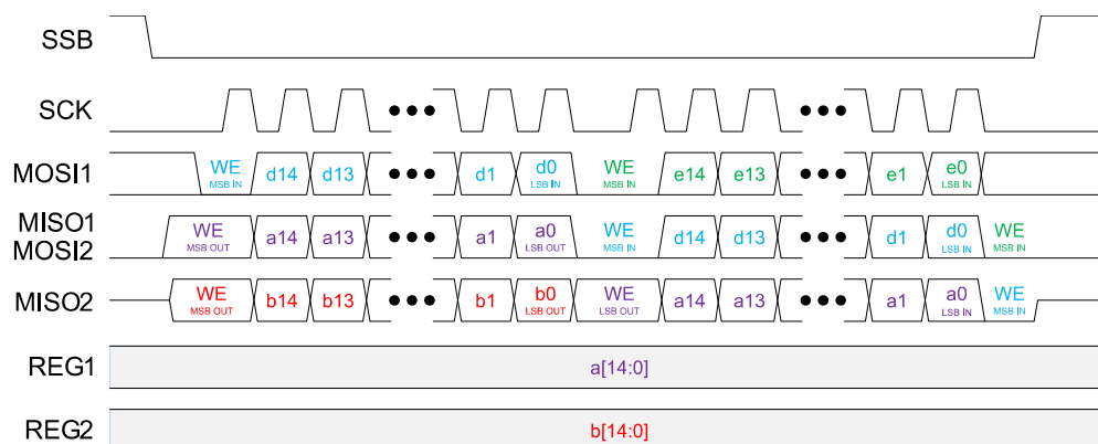
Figure 19. SPI with 2 ICs Daisy-chained
