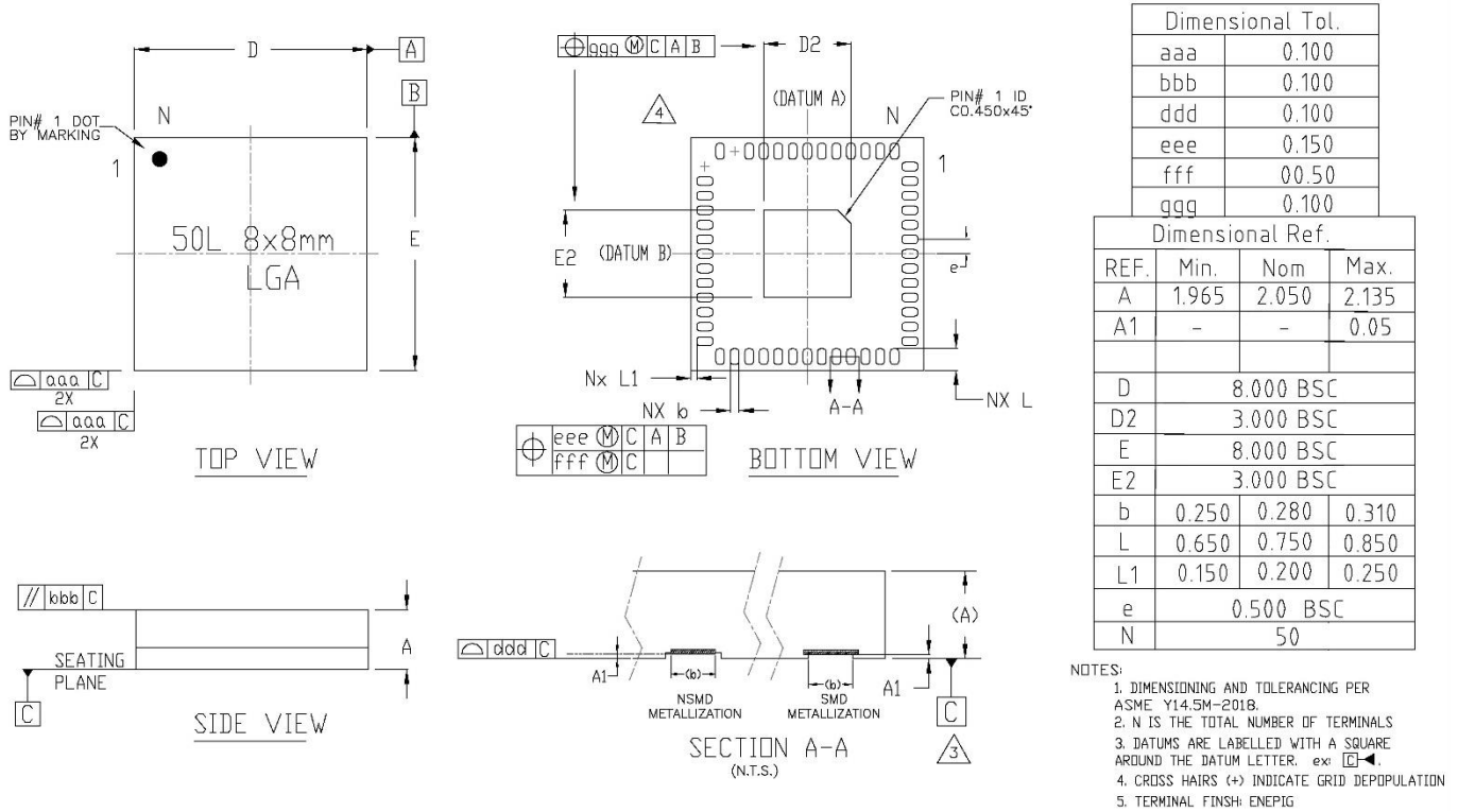
Figure 24. Package Drawing
