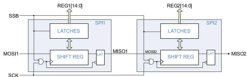
Figure 19. SPI with 2 ICs Daisy-chained
