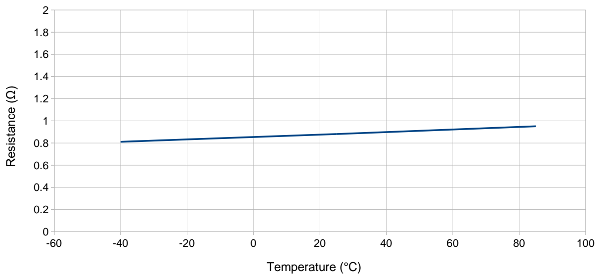
Figure 7. On-State Resistance over Temperature (Measured at 1A)
