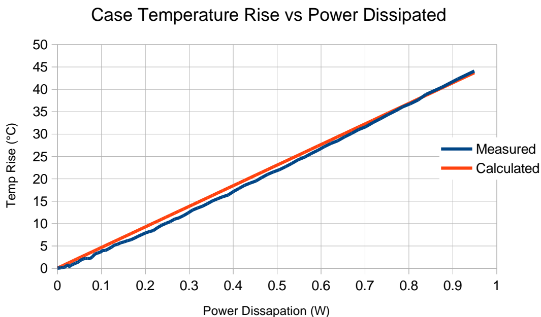
Figure 3. Case Temperature Rise versus Power Dissipated
