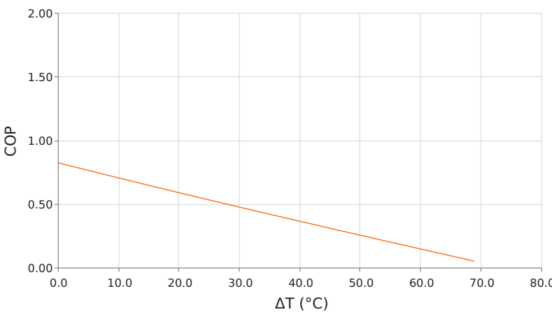
Coefficient of Performance (COP = Q_c/P_{in} ) T_{hot} = 35\text{ }^{\circ}\text{C} | I_{operating} = 5\text{ Amps}
