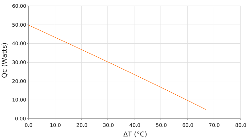
Heat Pumped at Cold Side ( Q_c ) T_{hot} = 35\text{ }^{\circ}\text{C} | I_{operating} = 5\text{ Amps}
