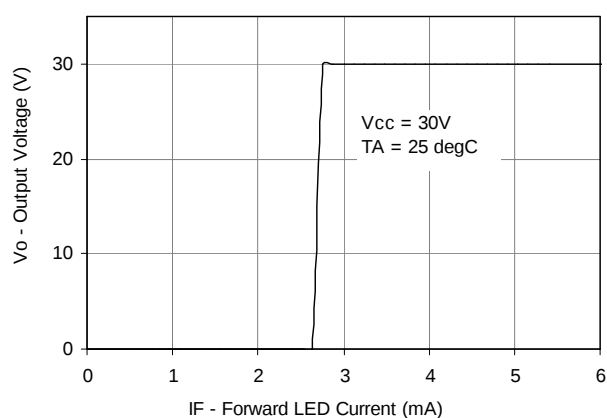
Figure 16: Transfer Characteristics
