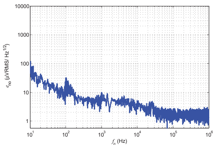
Figure 19: Output noise voltage spectral density
