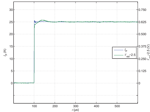
Figure 13: Step response
