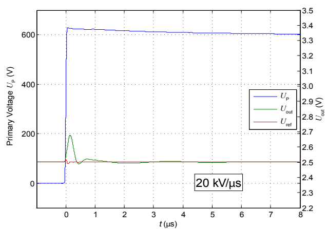
Figure 10: du/dt
