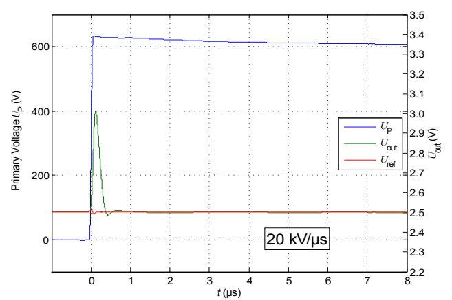
Figure 5: du/dt
