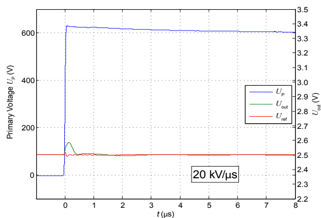
Figure 15: du/dt
