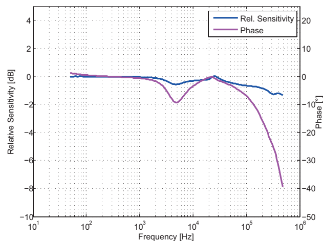
Figure 12: Frequency response
