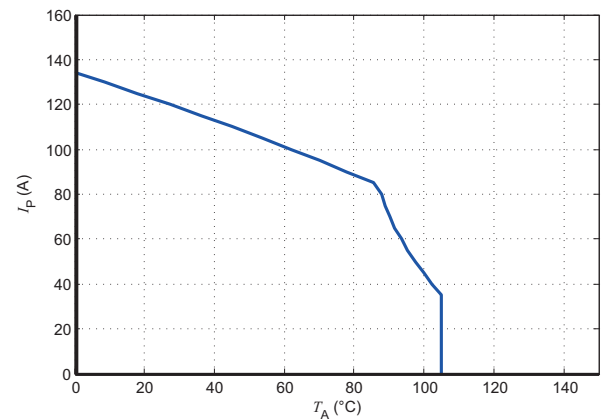
Figure 24: I_p vs T_A for LESR 50-NP
