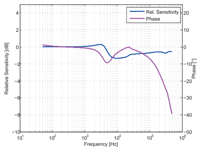
Figure 7: Frequency response
