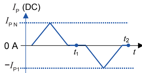
Figure 27: Current cycle used to measure magnetic and electrical offset (transducer supplied)
