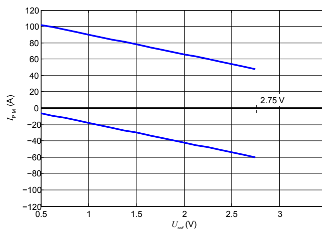
Figure 31: Measuring range versus external U_{ref} LESR 15-NP
