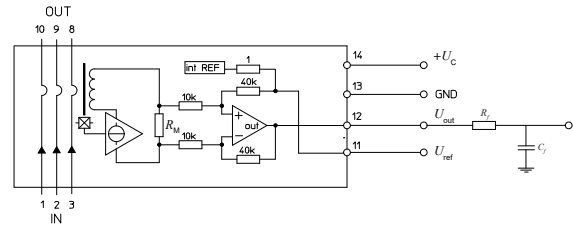
Figure 29: filtered U_{out} connection
