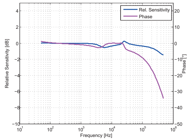
Figure 17: Frequency response
