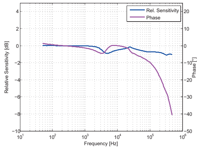
Figure 2: Frequency response
