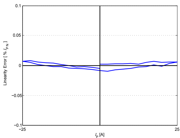
Figure 11: Linearity error
