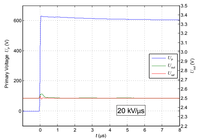
Figure 20: du/dt
