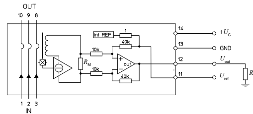
Figure 26: Test connection
