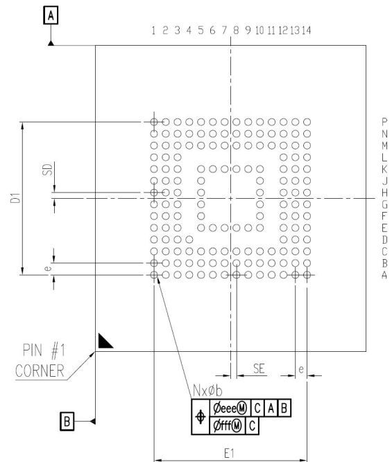
BOTTOM VIEW
