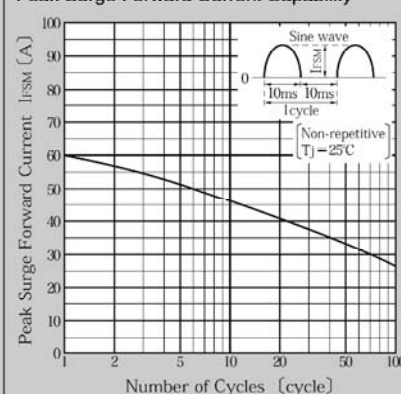
Peak Surge Forward Current Capability
