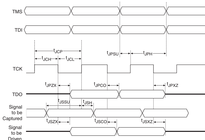
Figure 3-6. JTAG Timing Waveform for MAX V Devices
