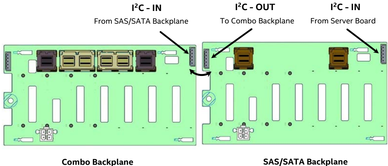
Figure 58. I²C connector Identification - Combo Backplane as the 2 nd Backplane Option
