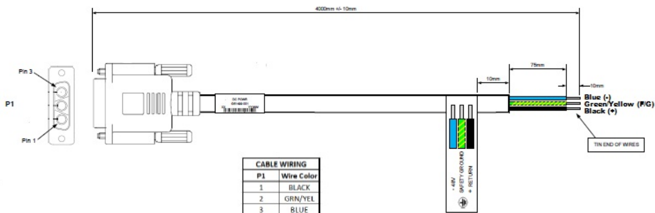
Figure 29. DC Power Cord Specification
