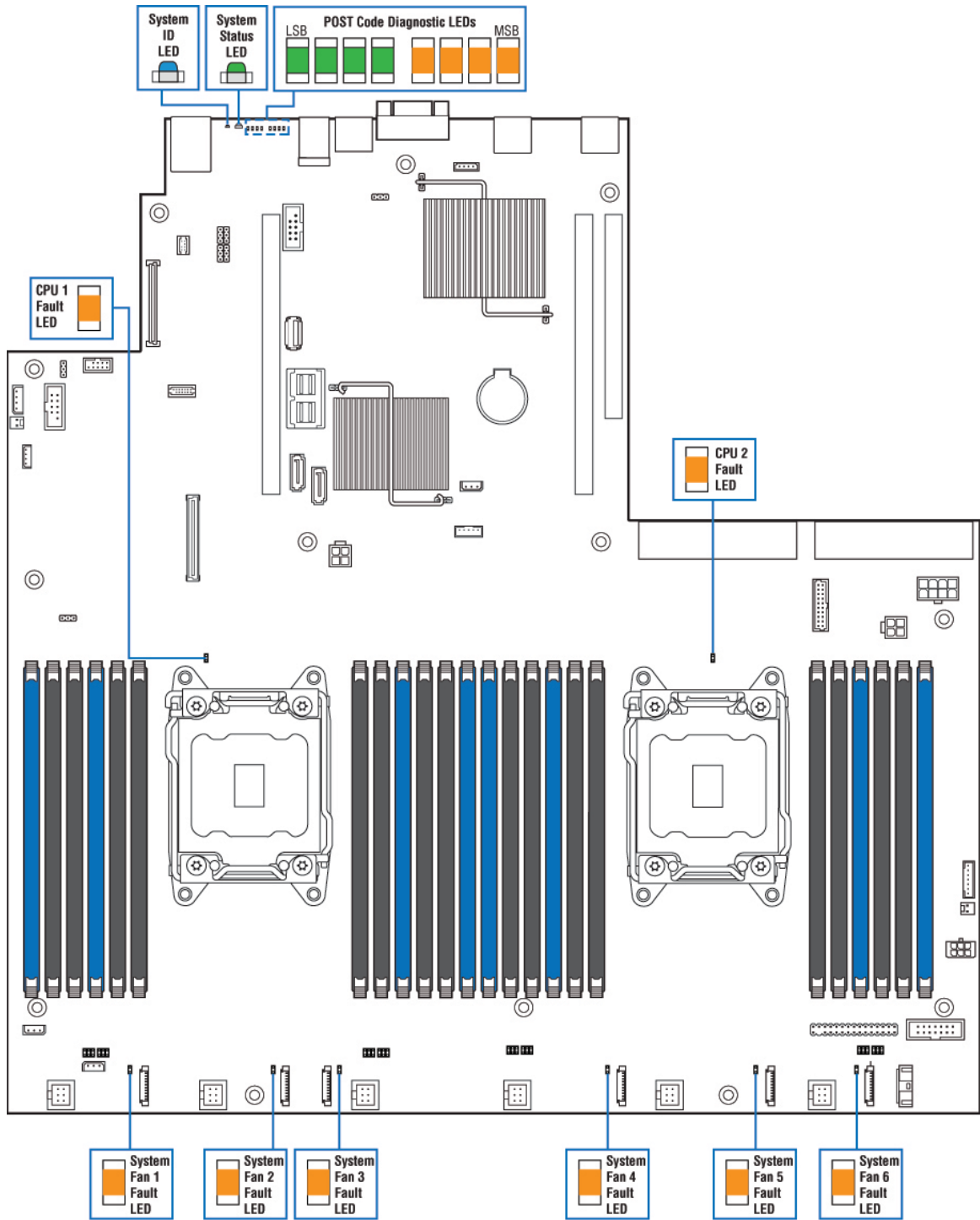
Figure 5. Light Guided Diagnostic LEDs
