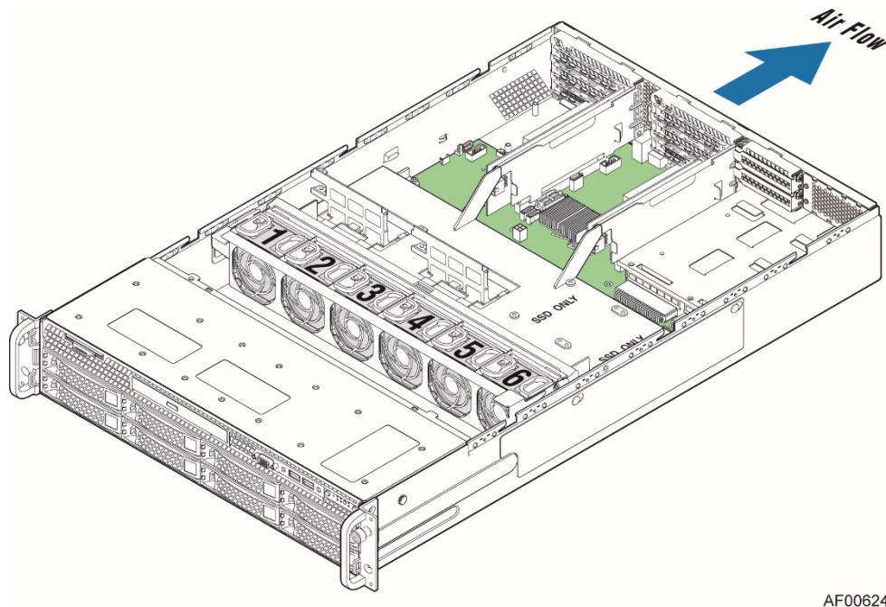
Figure 30. System Air Flow and Fan Identification
