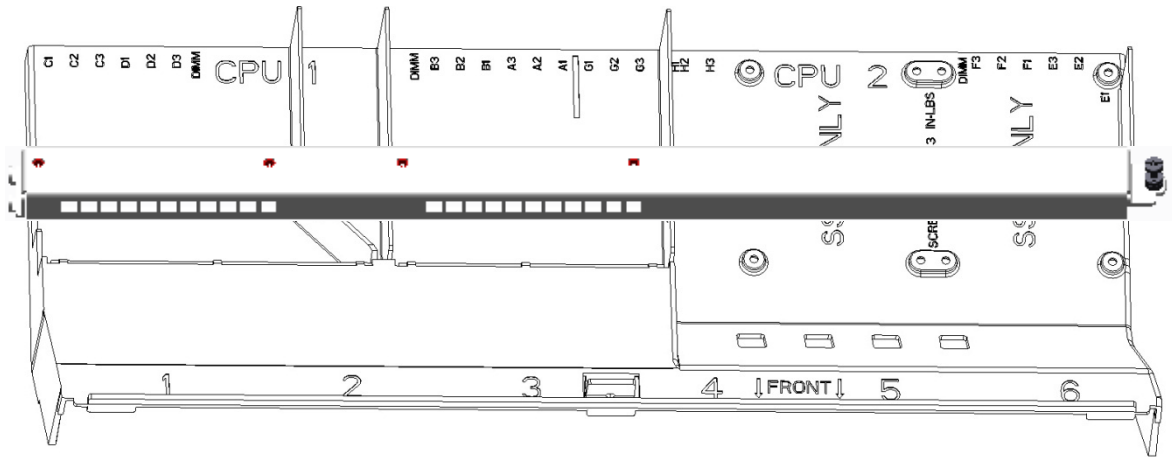
Figure 38. Shipping Bracket Placement
