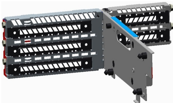
Figure 78. Left and Right Views of Riser Card #2 & #3 Bracket
