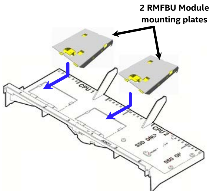
Figure 69. Dual RMFBU Mounting Bracket Installation
