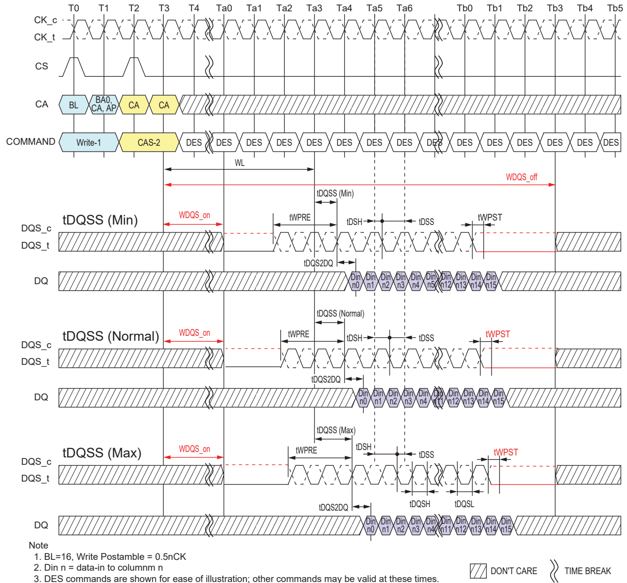
Figure 4.16 — Write Timing
