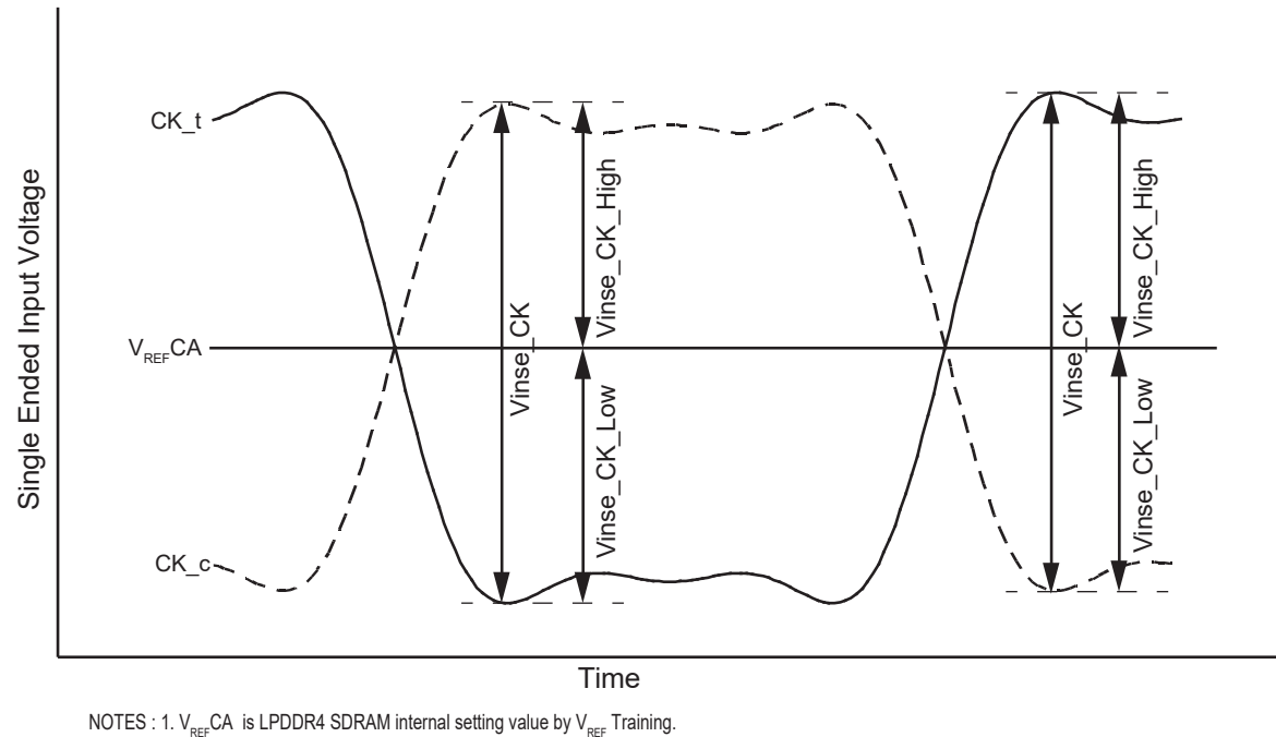
Figure 7.6 — Clock Single-Ended Input Voltage
