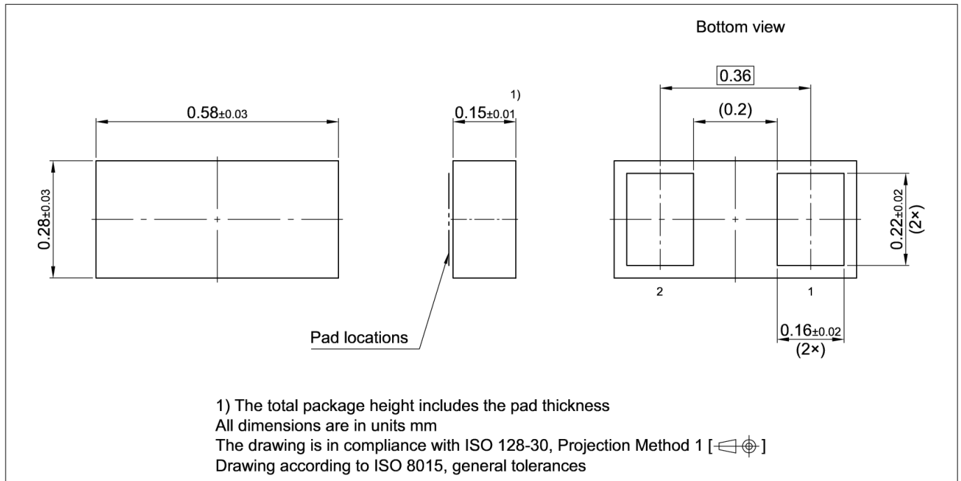
Figure 13 WLL-2-11 package
