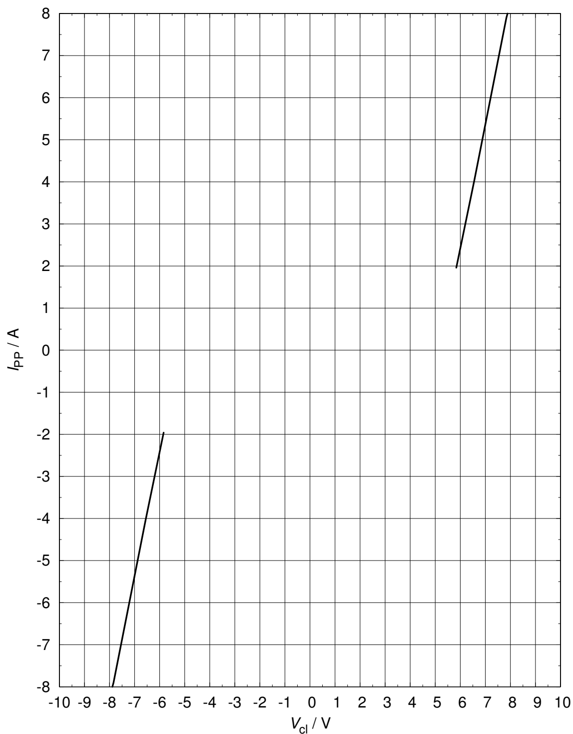
Figure 10 Clamping voltage (Surge): I_{PP} = f(V_{Cl}) , based on IEC61000-4-5
