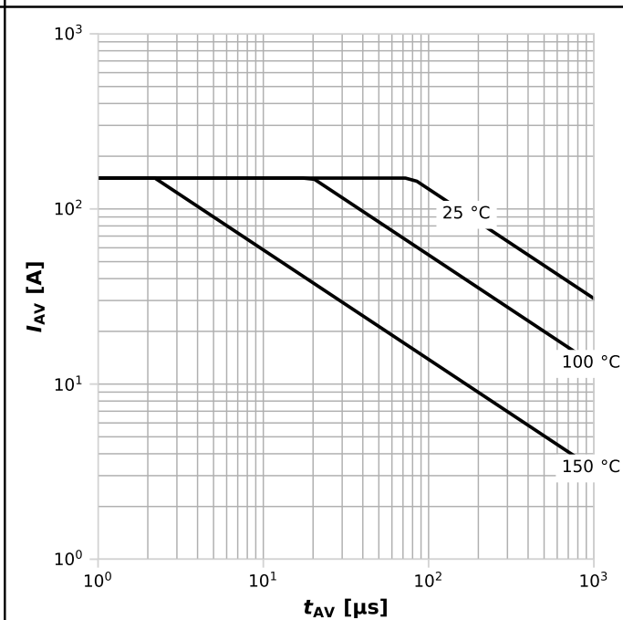
Diagram 14: Avalanche characteristics
