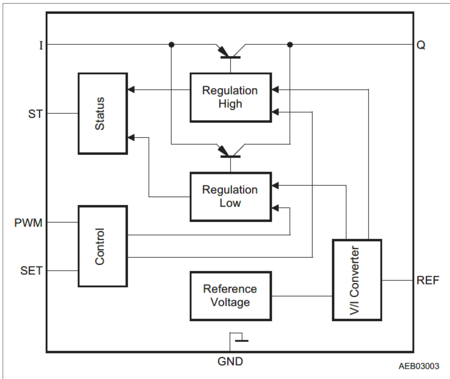
Figure 3 Block Diagram
