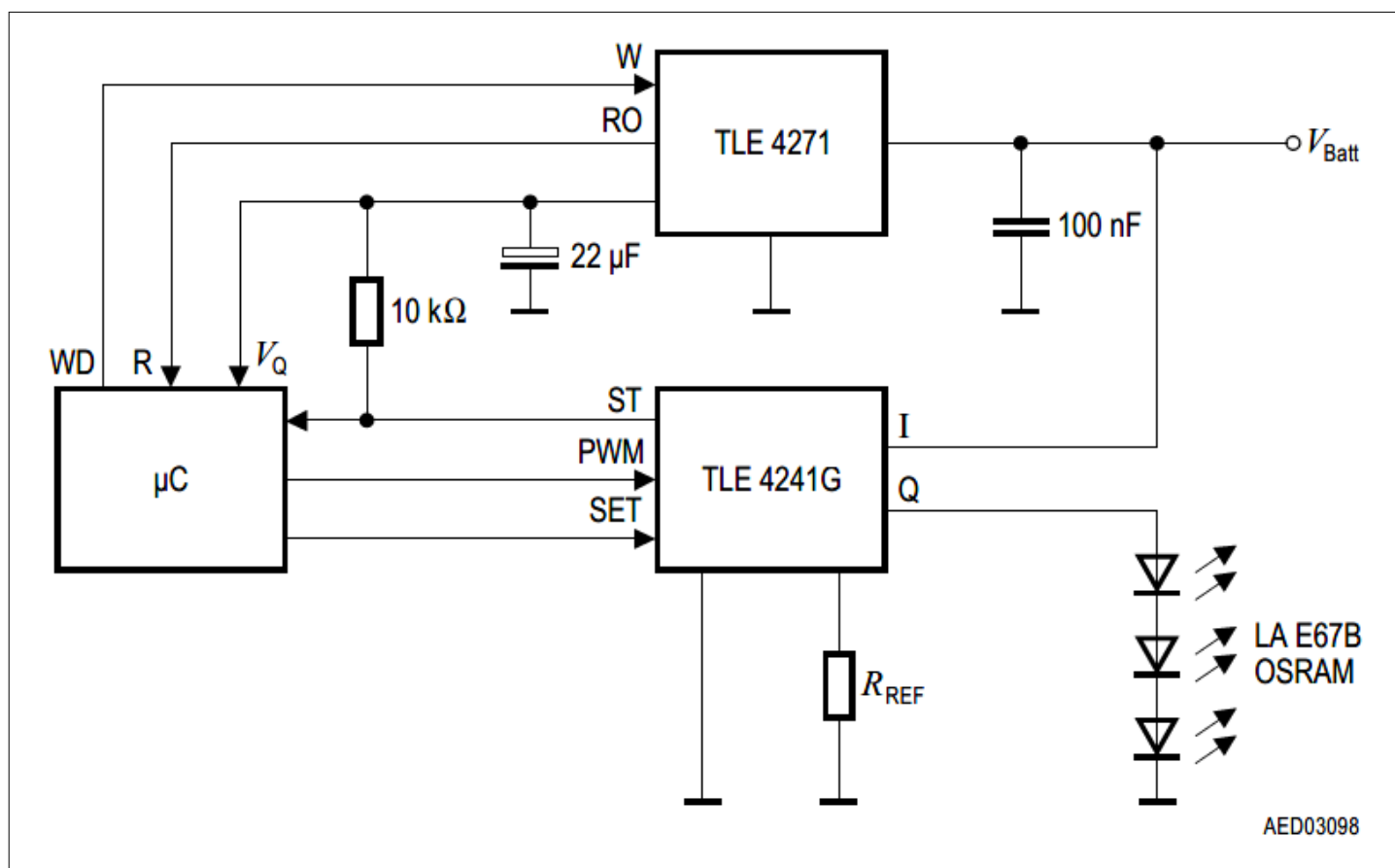
Figure 5 Application Circuit
