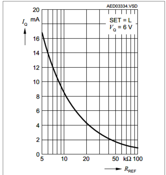
Figure 8 Output Current versus External Resistor, SET = L
