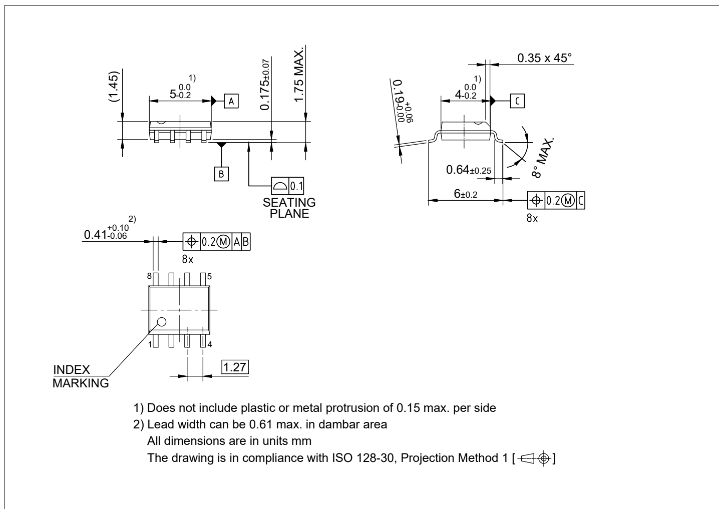
Figure 16 PG-DSO-8-16
