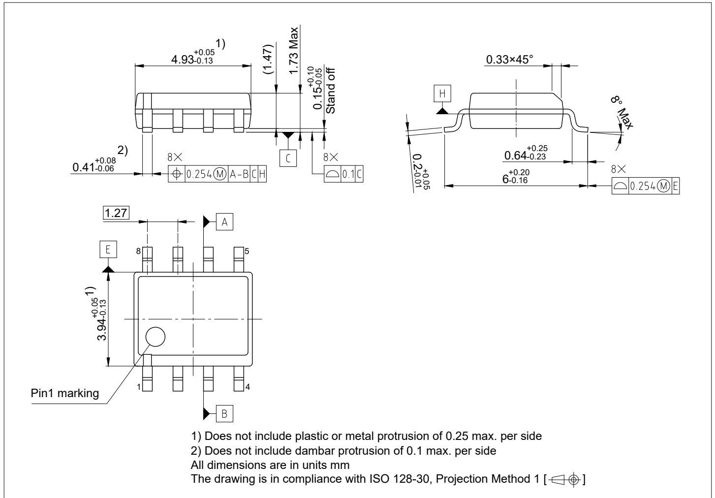
Figure 17 PG-DSO-8-62
