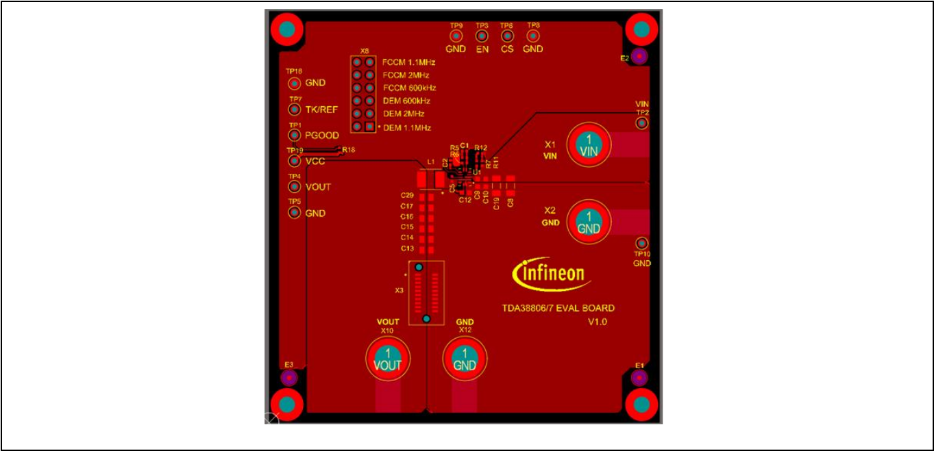
Figure 1 Top Layer
