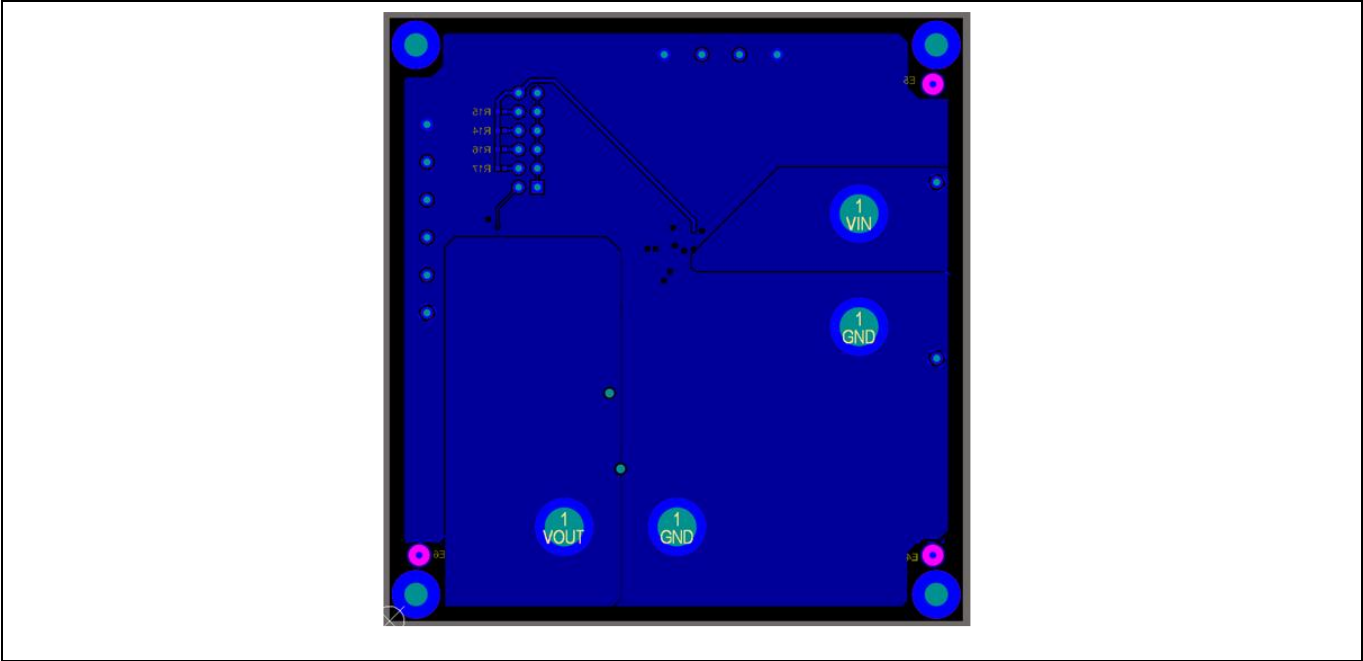
Figure 2 Bottom Layer
