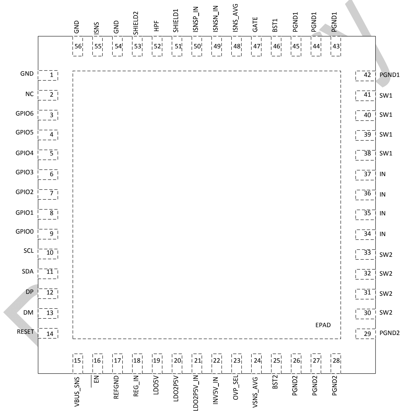
Figure 1. TQFN-56 7mmx7mm
