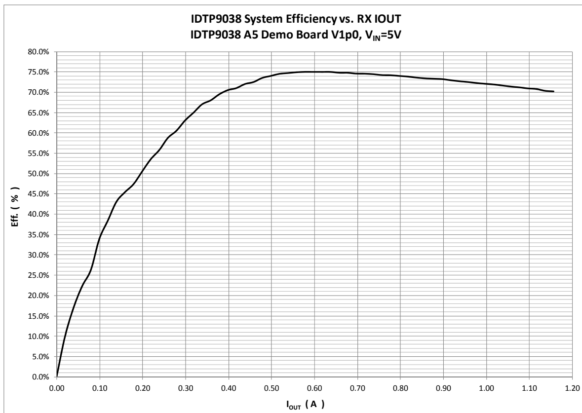
Figure 3. Efficiency vs RX Output Current, V_{IN}=5V
