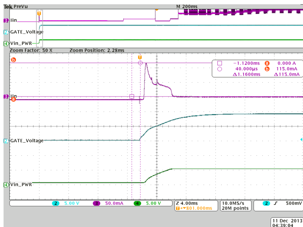
Figure 4. Inrush Current Limit Operation
