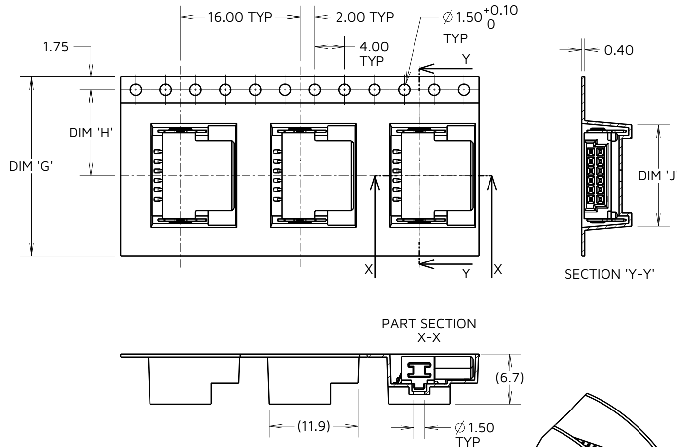
TAPE DETAILS FOR 12 TO 16 CONTACT CONNECTORS
