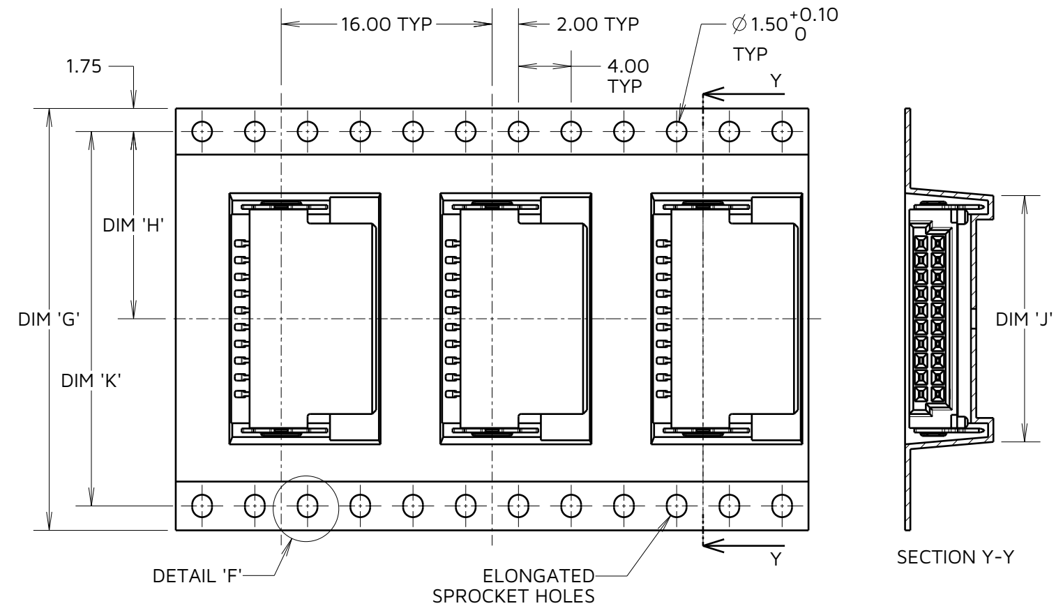
TAPE DETAILS FOR 20 TO 80 CONTACT CONNECTORS
