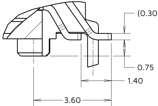
DETAIL 'F'
