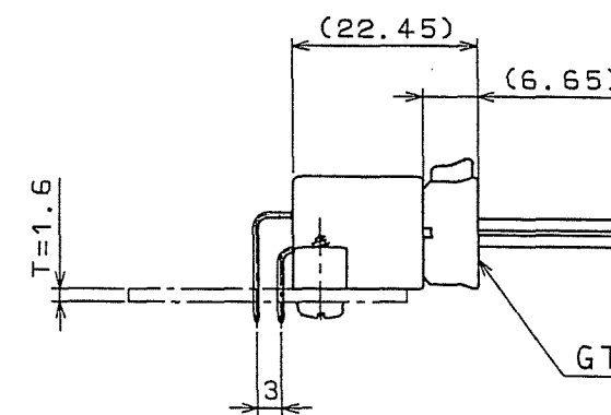
MATED CONNECTORS
