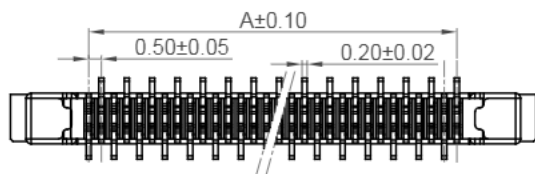
Right Footprint Version (Standard)
