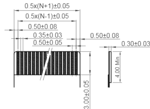
Recommended FFC/FPC Dimensions
