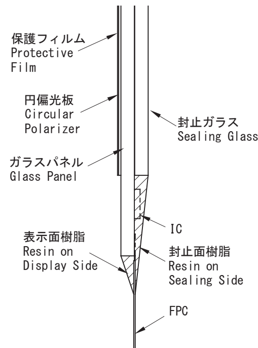
B部拡大図 (5 : 1) B-Portion Magnified Drawing (5:1)
