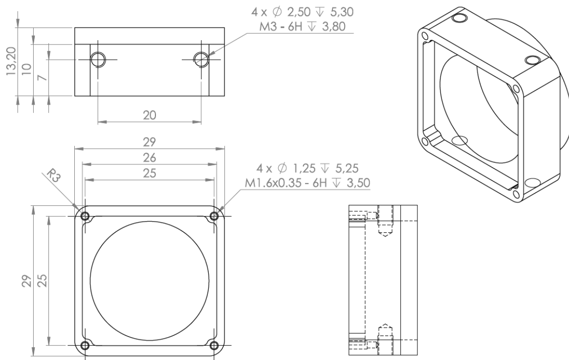
Figure 24: CS-Mount Body for 28 mm FSM
