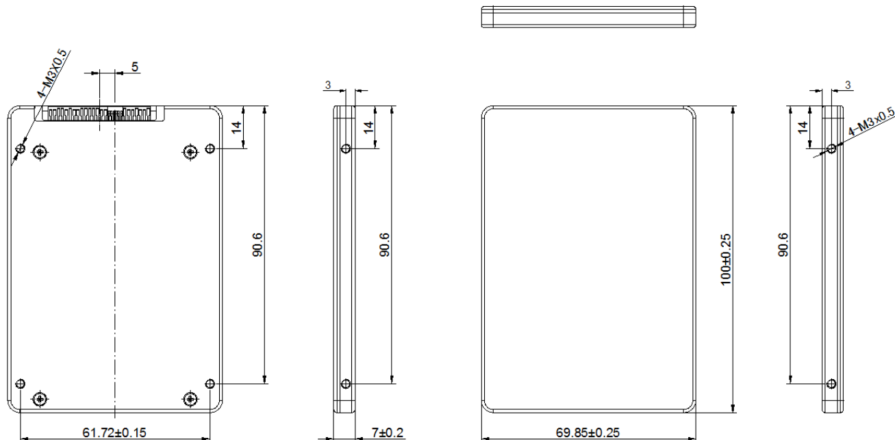
Figure 2: U.2 physical dimension diagram
