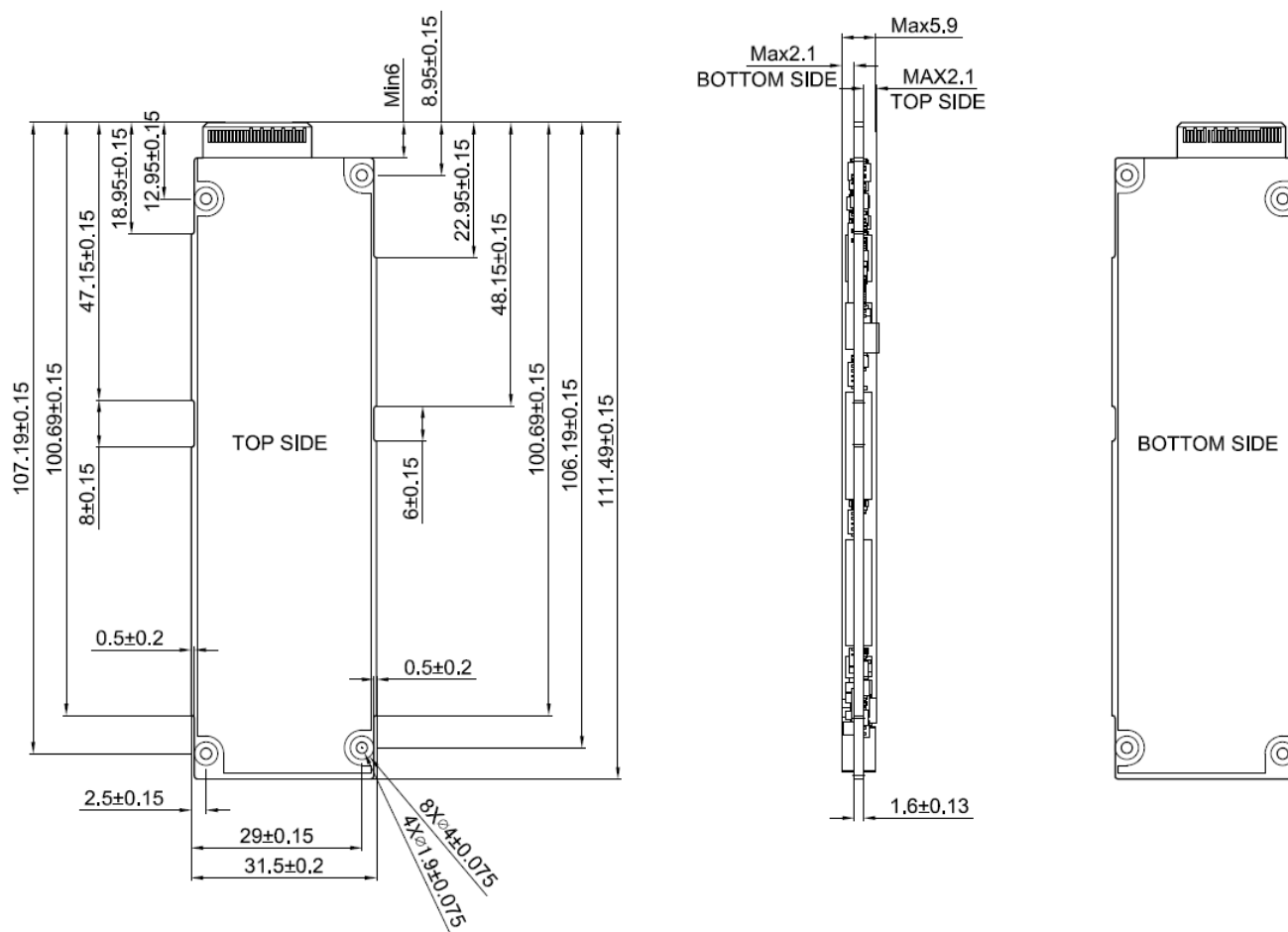
Figure 4: E1.S physical dimension diagram
