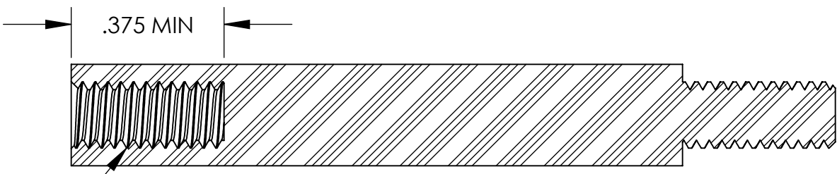
8-32 THREADS SECTION A-A
