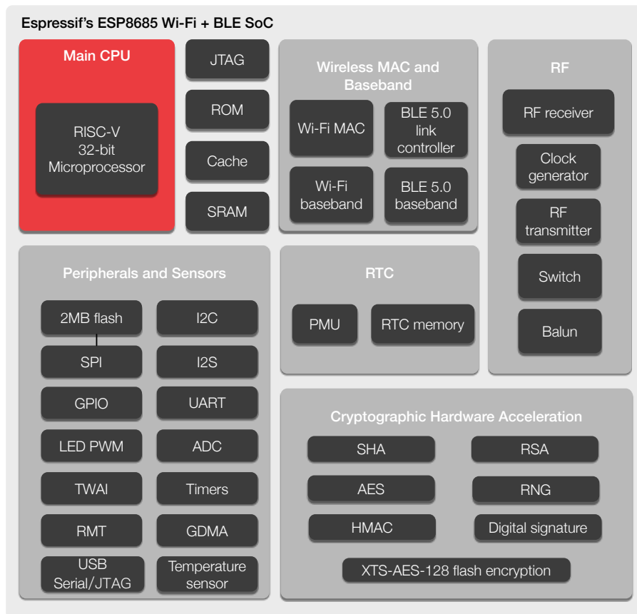
Figure 1: Block Diagram
